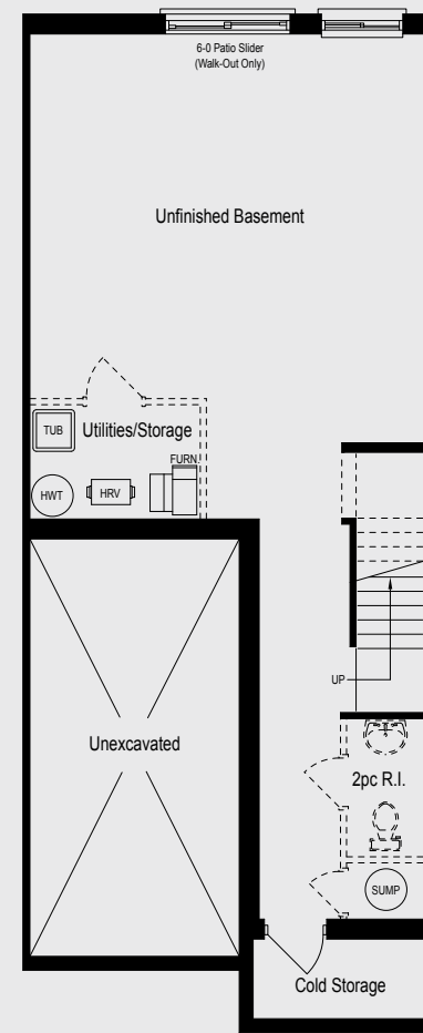
BASEMENT INTERIOR UNIT
