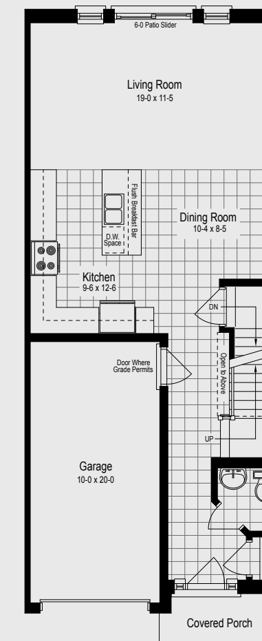
MAIN FLOOR INTERIOR UNIT
